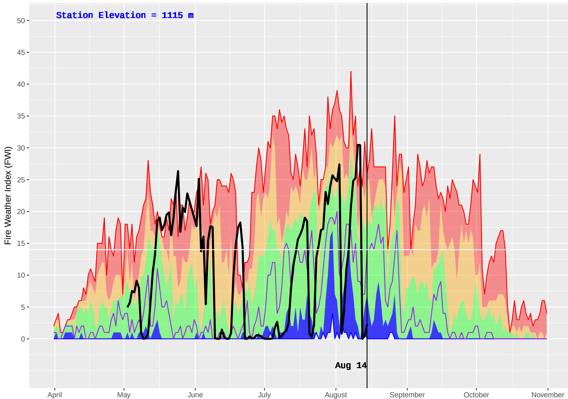
SICAMOUS (882) : Historical (2004–2016) and Current (2018) Daily Fire Weather Index (FWI)
