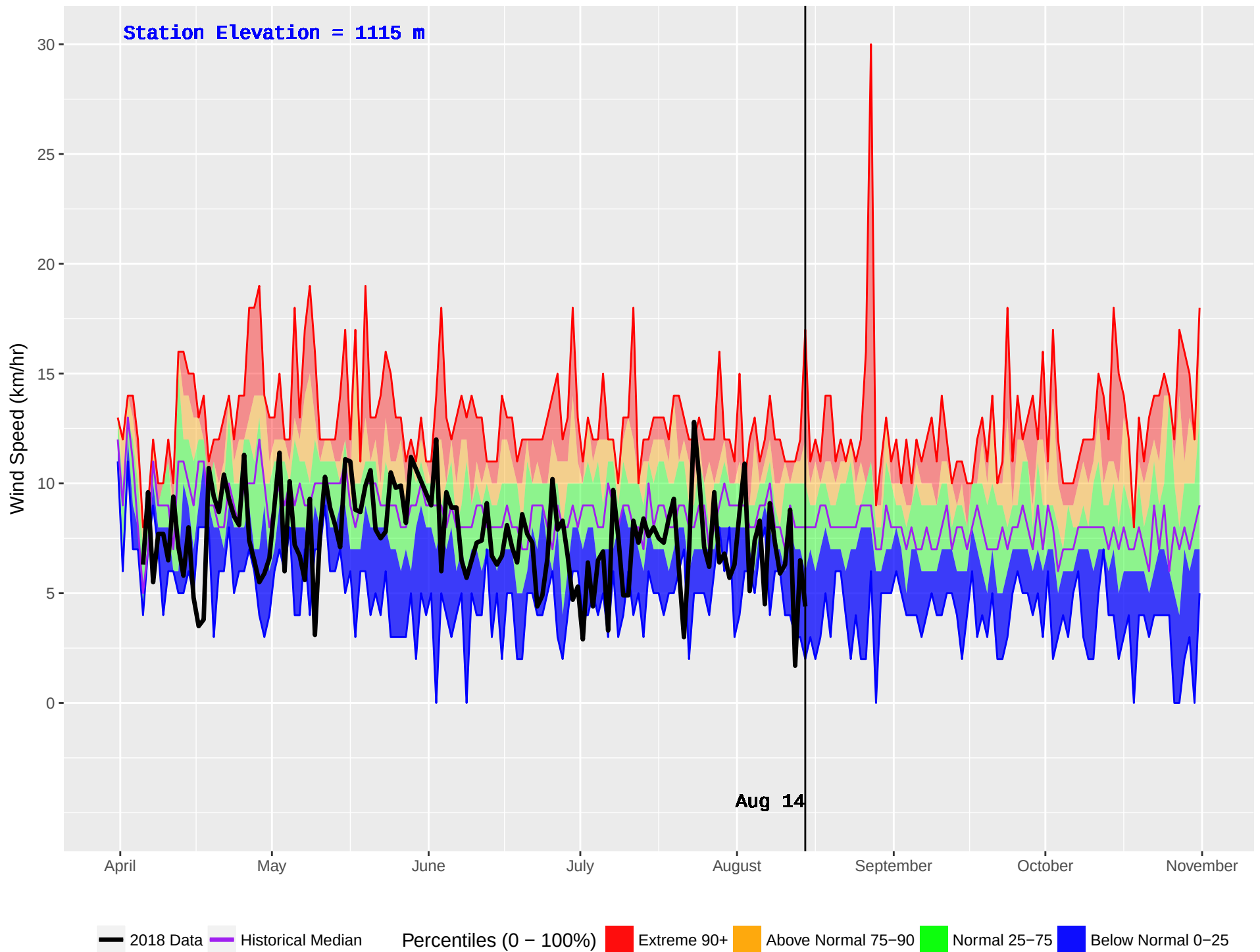
SICAMOUS (882) : Historical (2004–2016) and Current (2018) Daily Wind Speed
