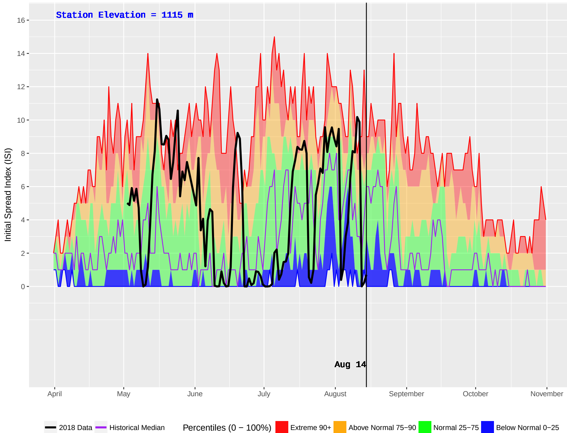
SICAMOUS (882) : Historical (2004–2016) and Current (2018) Daily Initial Spread Index (ISI)
